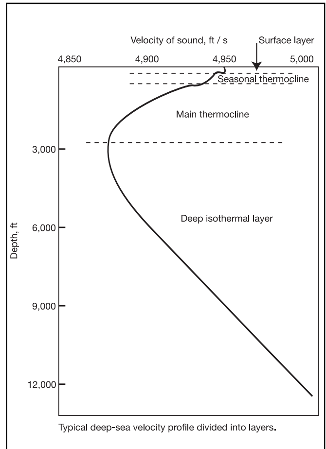
Fig. 5 This graph illustrates the velocity variations of sound in water due to density variations in the sea. As the ocean gets deeper, the pressure rises increasing the density, and thus the velocity. This is the case in the “deep isothermal layer.” The velocity of sound in the “main thermocline” area changes dynamically due to long term climate changes and turbulence caused by global currents. The “seasonal thermocline” varies dynamically over seasons and due to deep weather generated turbulence. Finally the speed of sound in the “surface layer” varies due to diurnal temperature changes and surface turbulence.
