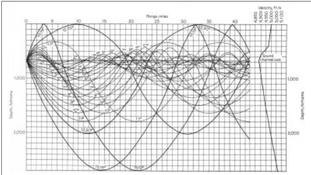
Fig.4 Sound Channel: The sound will tend to focus around the sound channel axis. We start noticing a channel adherence as the angle approaches 10 degrees. But as the angle of incidence approaches 0 degrees, it really follows the axis.
